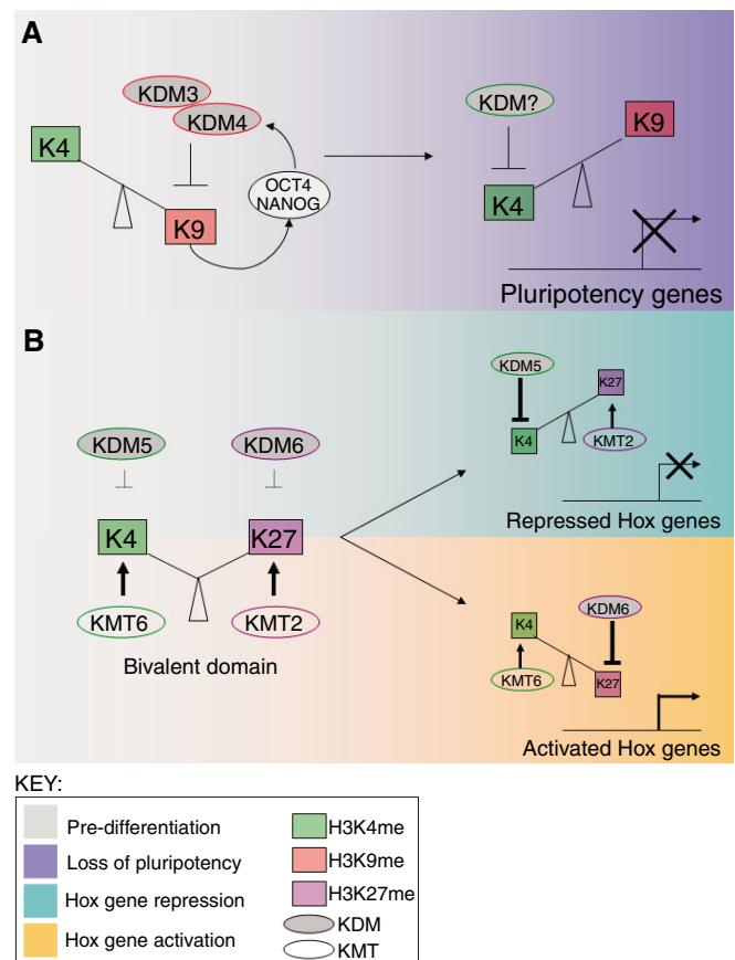
Fig. 2. Opposing histone demethylases regulate developmental genes.
