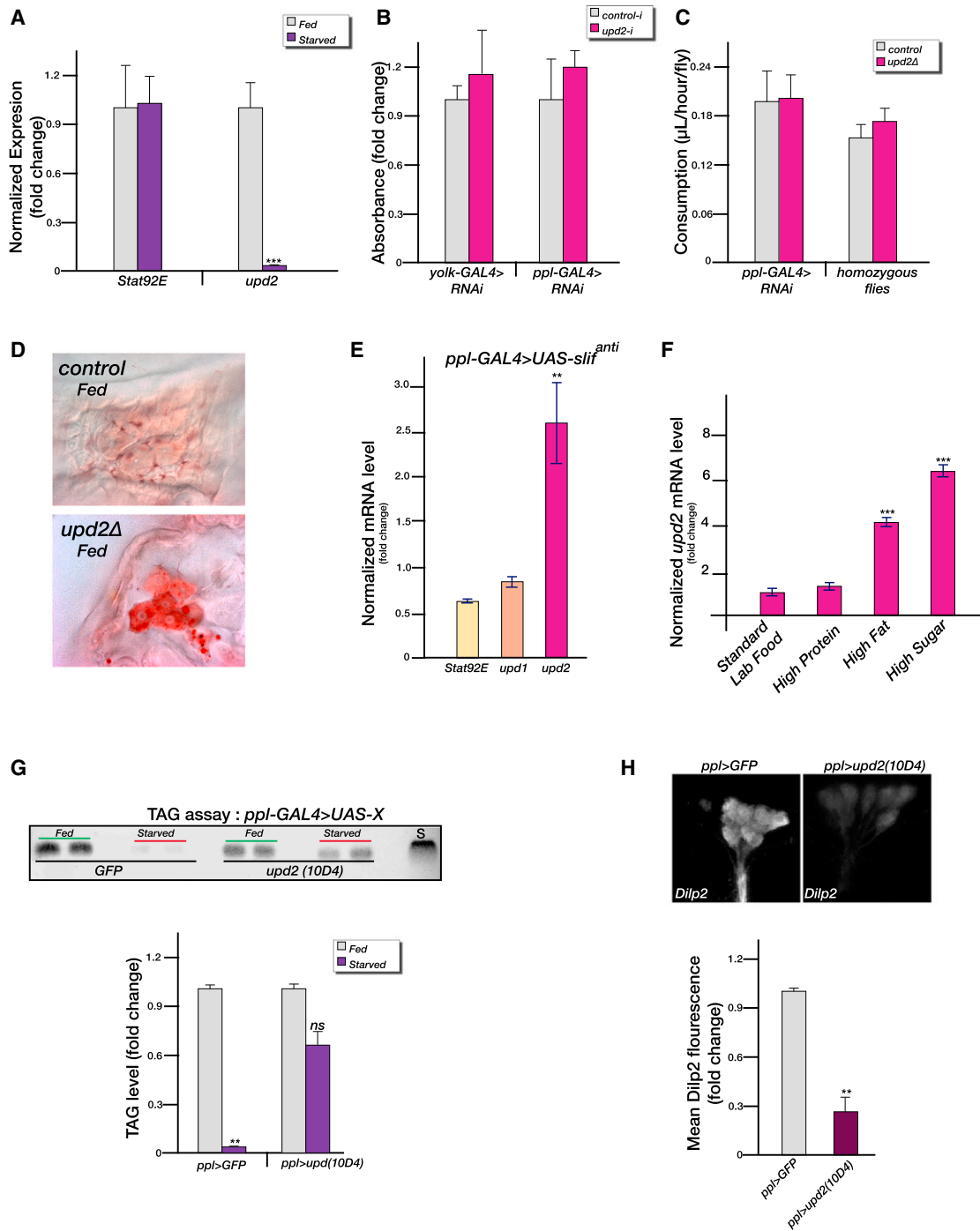
Figure 2. Upd2 Expression in the FB Signals the Fed State
